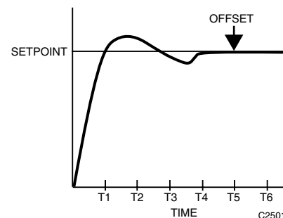
Fig. 40. Proportional-Integral-Derivative Control.
