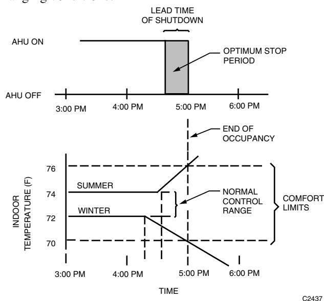
Fig. 6. Optimum Stop.
