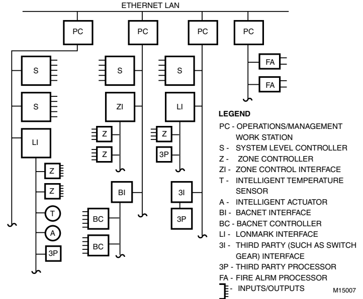
Fig. 11. In-Depth Integrated System.
