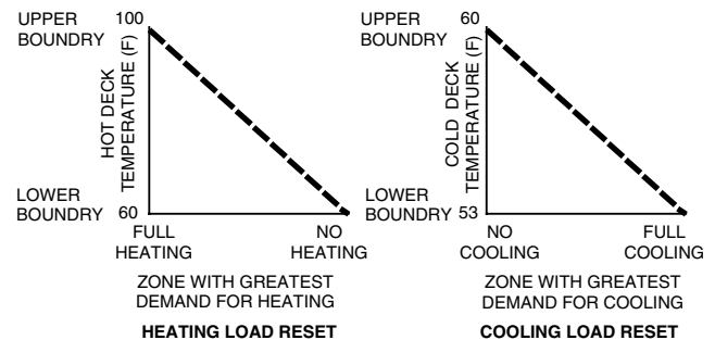
Fig. 9. Typical Load Reset Schedules.
