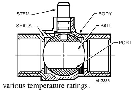
Fig. 3. Ball Valve.
