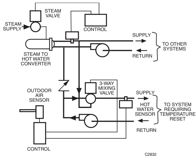
Fig. 84. Hot Water Converter Control with Constant Temperature and Reset Zones.
