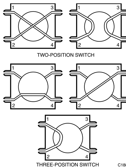
Fig. 54. Pneumatic Switches.
