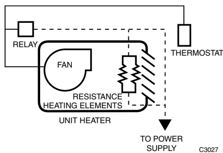
Fig. 16. Unit Heater Two-Position Control—Electric Heat.
