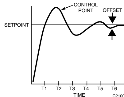
Fig. 39. Proportional-Integral Control.
