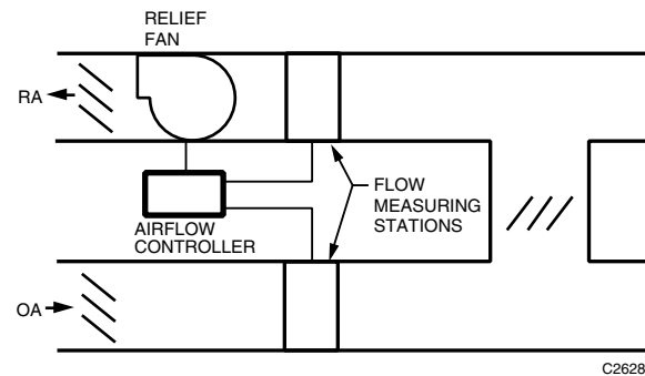
Fig. 33. Airflow Tracking Control for Relief Fan.
