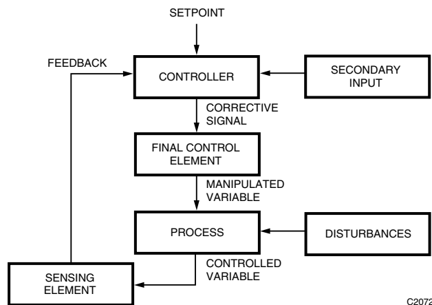
Fig. 19. Feedback in a Closed-Loop System.
