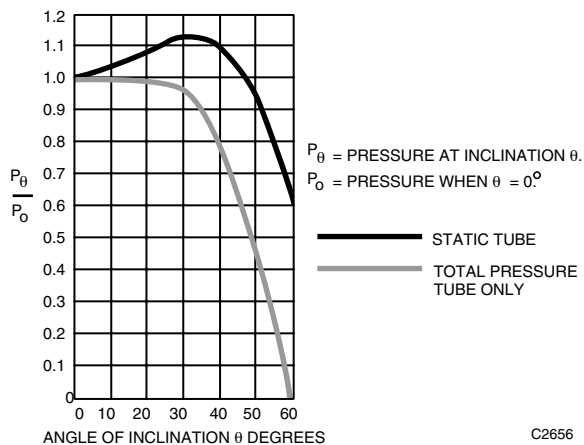
Fig. 16. Error Caused by Improperly Mounting Pitot Tube in Airstream.
