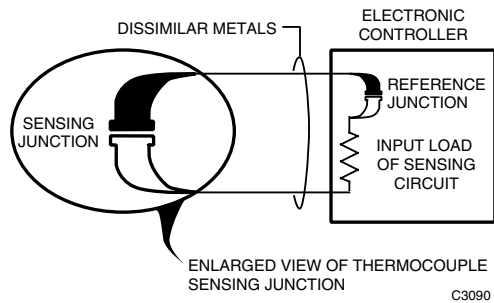
Fig. 7. Basic Thermocouple Circuit.
