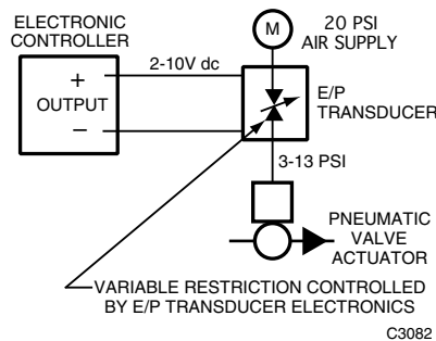
Fig. 19. Electric-to-Pneumatic Transducer.
