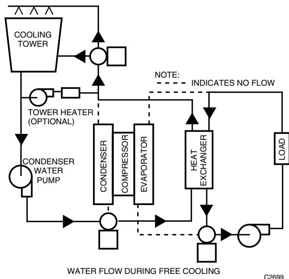
Fig. 34. Free Cooling Using Auxiliary Heat Exchanger.
