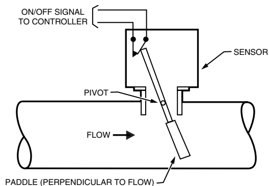
Fig. 53. Paddle Flow Sensor.
