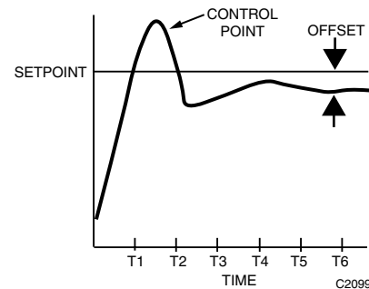
Fig. 38. Proportional Control.
