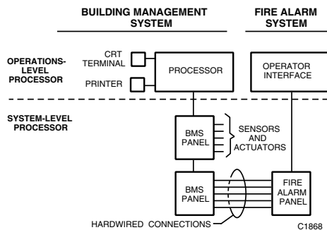
Fig. 10. Surface Integrated System.
